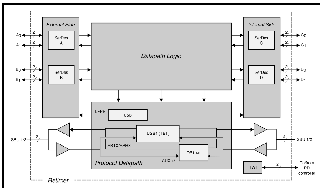
Fig. 1: Functional KB8002 block diagram
